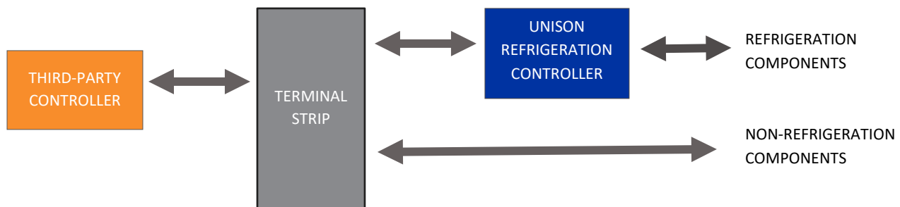
Figure 1: Third-party controller with Unison Controls Lite
